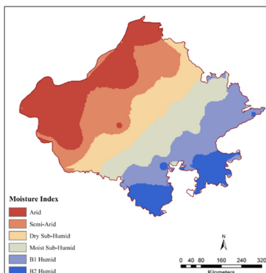
Figure 3(b): Thornthwaite's Humidity Provinces during 1981-2010 (Based on Thornthwaite (1948))
